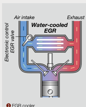
3 EGR cooler
